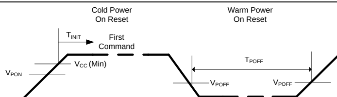
Figure 5.1 V CC Ramp Up and Ramp Down
