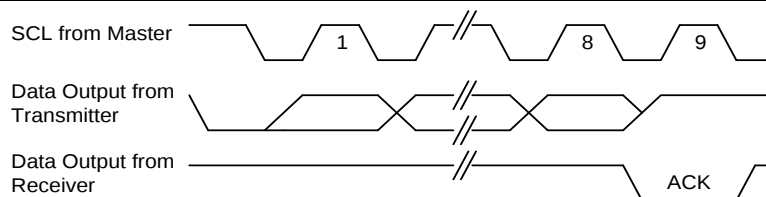
Figure 5.5. Output Acknowledge
