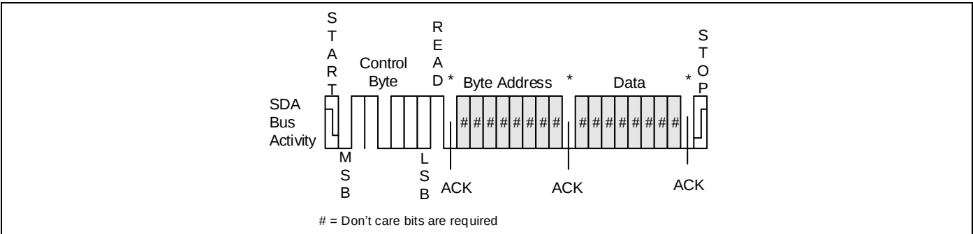
Figure 6.7 Read Write Protection Status; Read Page Address
