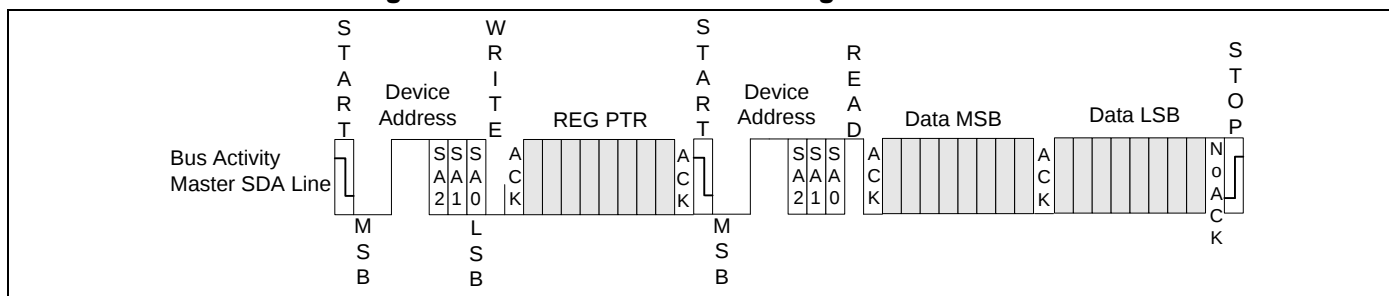
Figure 7.4 I2C Bus Pointer Write Register Word Read
