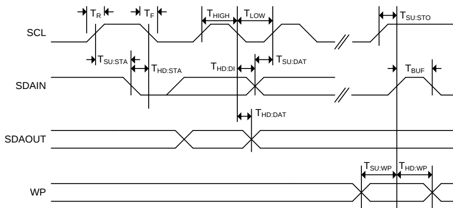
Figure 5.6. Bus Timing
