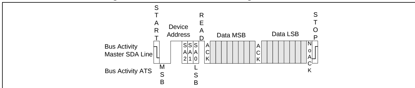
Figure 7.3 I2C Bus Preset Pointer Register Word Read
