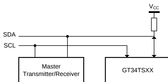
Figure 5.2. Typical System Bus Configuration
