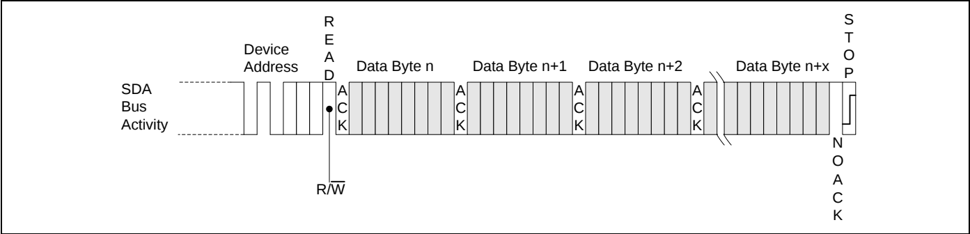
Figure 6.5 Sequential Read
