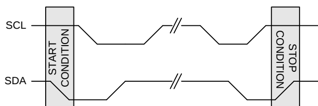
Figure 5.3. Start and Stop Conditions
