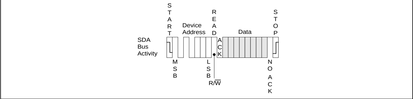
Figure 6.4 Current Address Read
